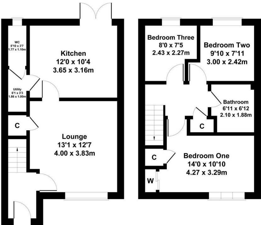
GROUND FLOOR
